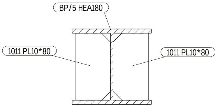
A - A 1:5
